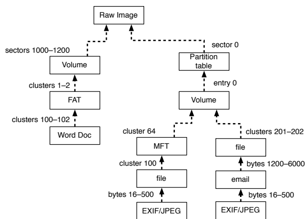
Figure 1: A diagramed version of a DEX description of evidence.
