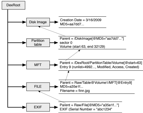
Figure 2: A diagram of the DEX file that appears in Appendix A. Solid lines represent enclosed elements. Dotted lines show the destination of Parent pointers.
